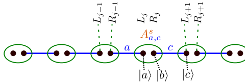
Figure 36: MPS representation of the AKLT valence-bond solid state (see also Fig. 4). The figure represents the index convention used in Eq. (107).
